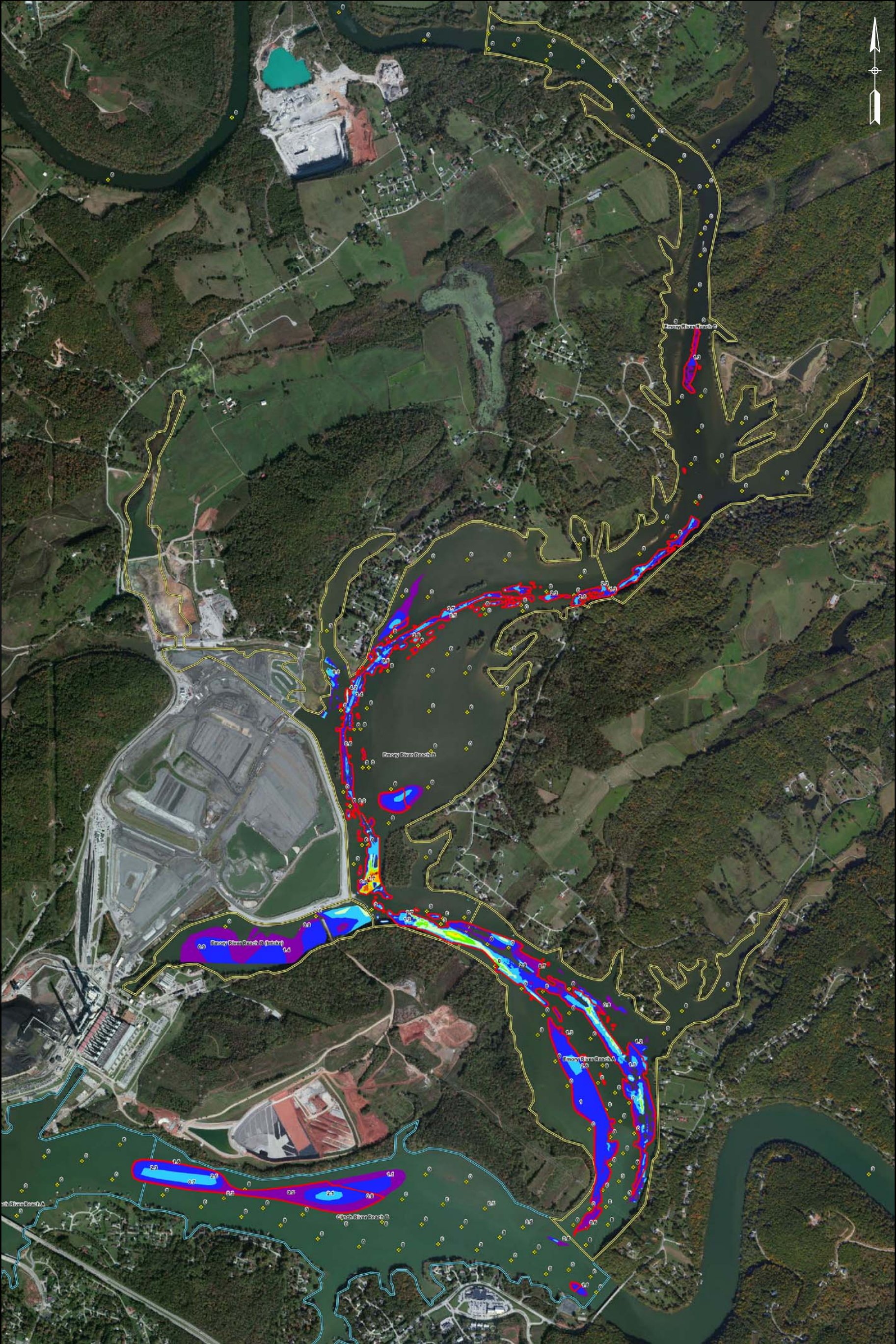
FIGURE 35 ALTERNATIVE 2B: TARGETED CAPPING KINGSTON ASH RECOVERY PROJECT
