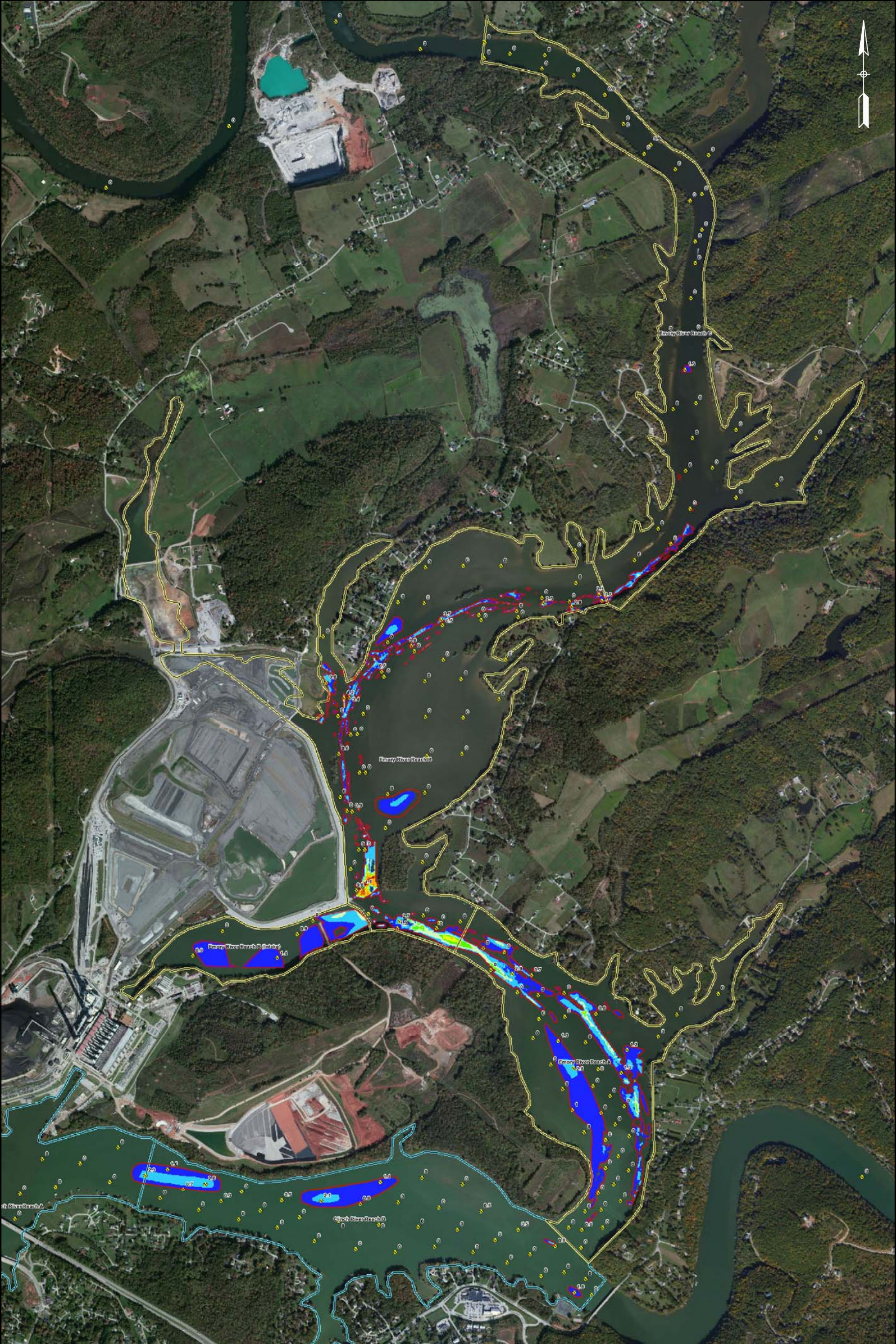
FIGURE 36 ALTERNATIVE 3A: DREDGING KINGSTON ASH RECOVERY PROJECT
