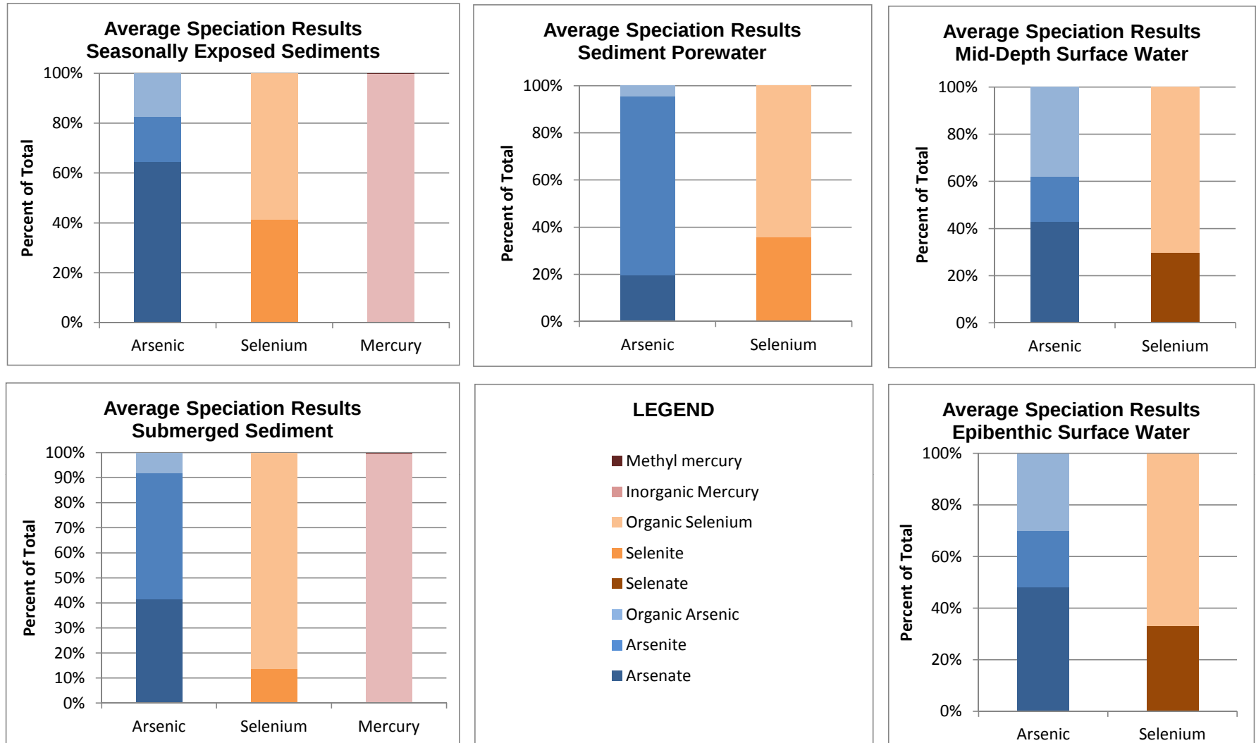
Figure 11. Average Speciation Results Multiple Media - All River Reaches
