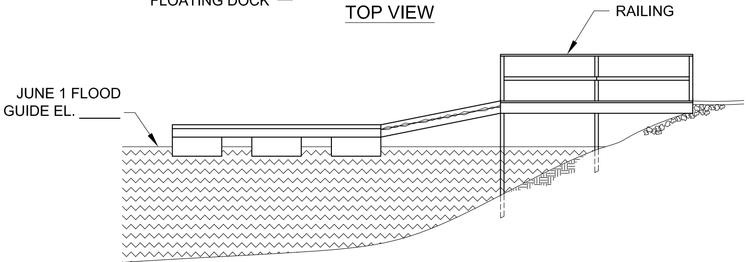
SIDE VIEW
