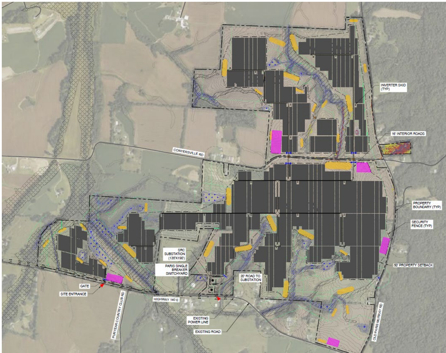
Figure 2.2-2 Project Site Layout Map
