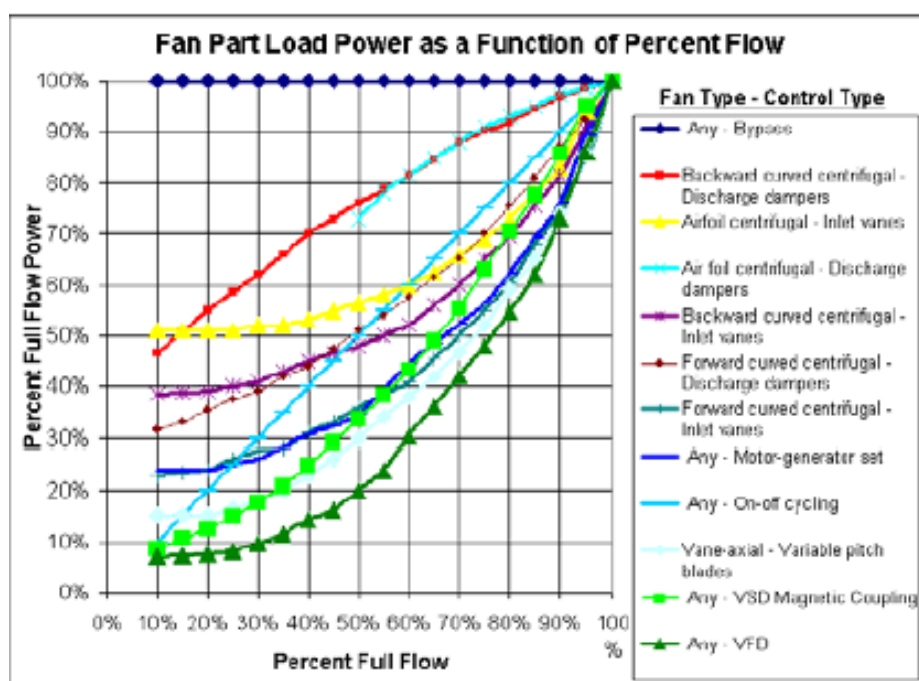
Figure 2. Fan Part Load Power as a Function of Percent Flow 258
