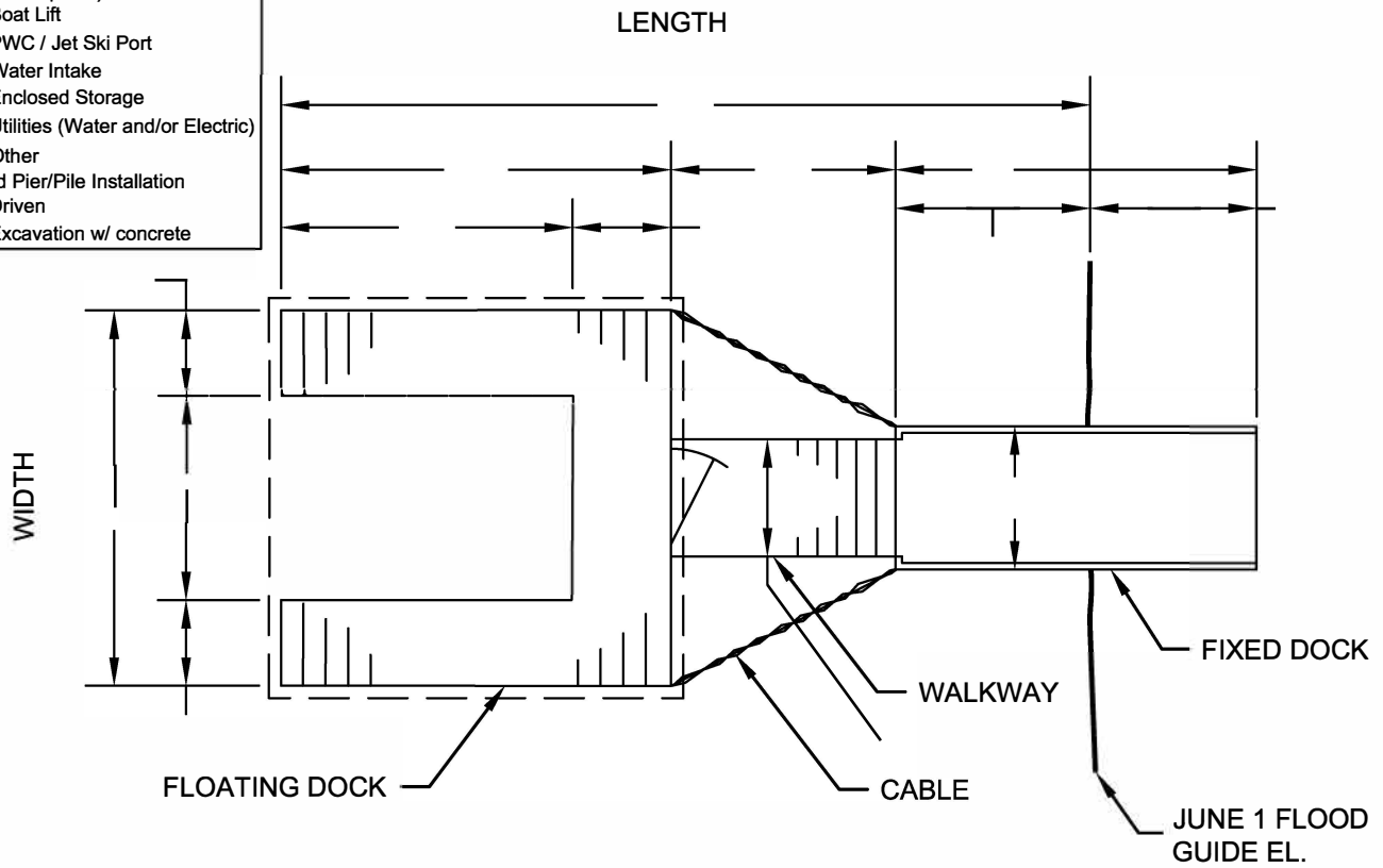
TOP VIEW
