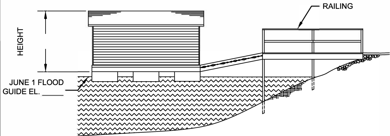
SIDE VIEW
