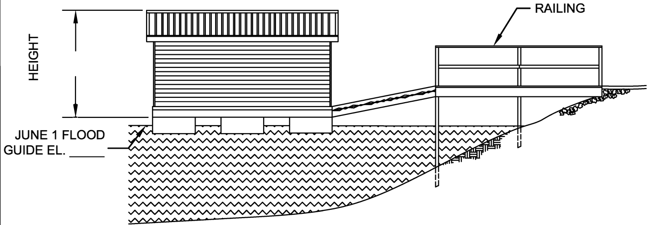
SIDE VIEW
